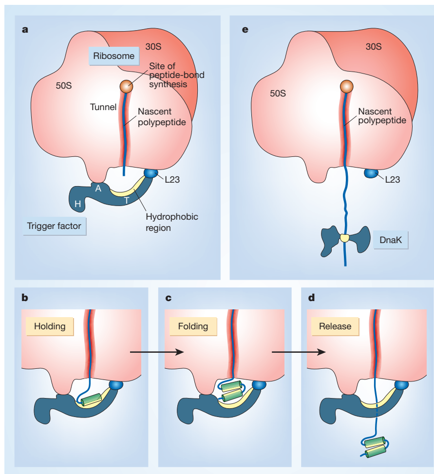
Figure 1 Chaperones at the ribosome. a , Ferbitz et al. 3 have determined the crystal structure of the trigger-factor tail domain (T) in complex with a ribosome large subunit (50S), and used this to position their crystallographic model of intact trigger factor, including the arm (A) and head (H) domains. Trigger factor forms a cavity, with a hydrophobic lining, at the exit of a tunnel in the ribosome from which newly made polypeptide chains emerge. Its main contacts are with the ribosomal protein L23. b–d , How the nascent polypeptide might behave. b , ‘Holding’, where hydrophobic sections (yellow) of the nascent structure (here on an \alpha -helix, symbolized by a barrel) could be stabilized by binding to trigger factor’s hydrophobic surface. c , ‘Folding’, where a further stretch of emerging chain docks with that of the first, forming a substructure within the cavity. d , ‘Release’, where the substructure dissociates from trigger factor, by an unknown mechanism, and a new segment of chain enters the cavity. e , The binding of nascent polypeptide chains by chaperone DnaK is entirely different, and involves a narrow hydrophobic arch in DnaK 9 (only the peptide-binding domain of DnaK is shown). The nascent chain might also acquire \alpha -helical structure within the ribosomal tunnel 12,13 , but this is not shown here.
